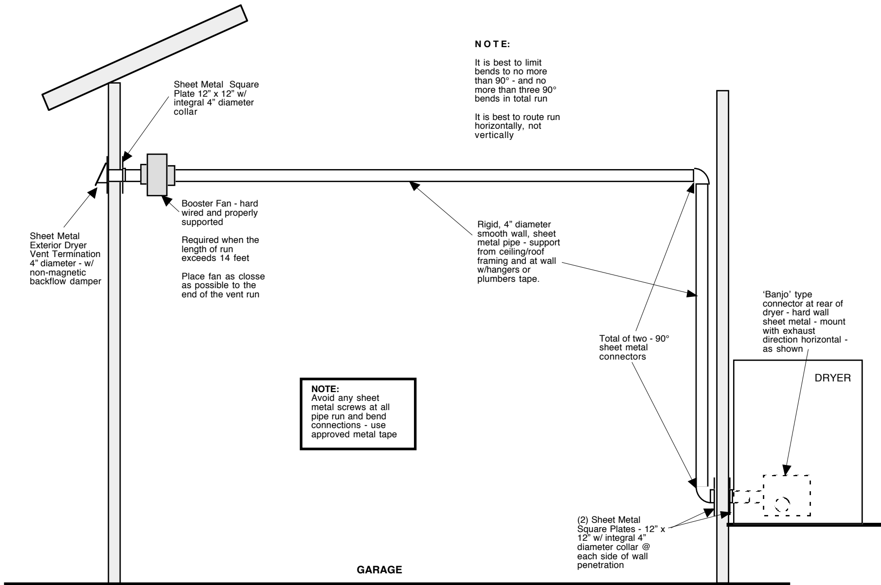
Schematic: Dryer Vent Run/Transitions/Termination - w/Booster Fan (when length of run exceeds 14 feet)
